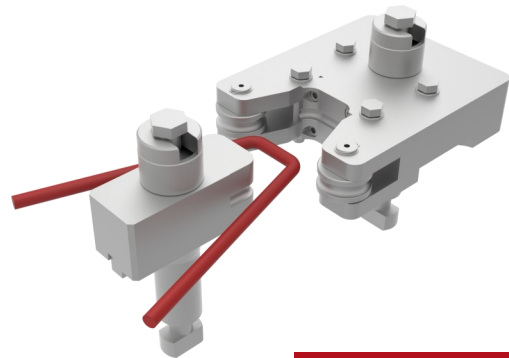
2-JAW bender
